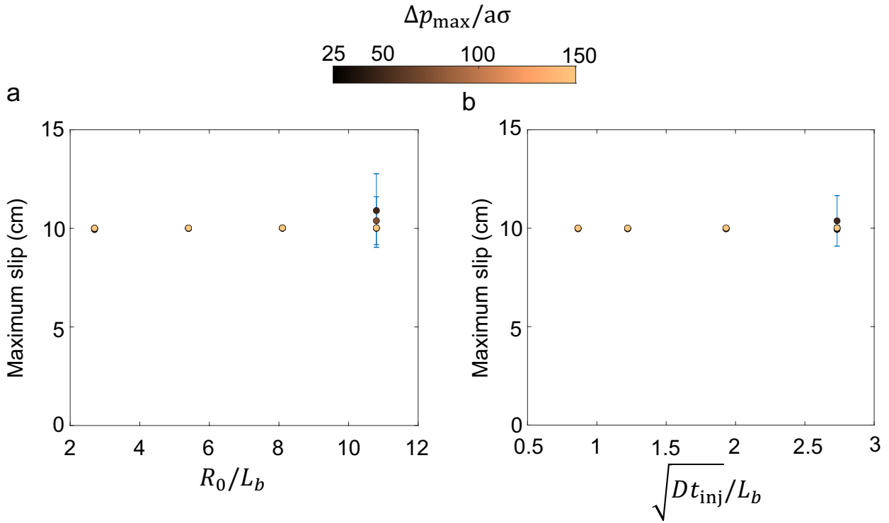
Figure S3. Average maximum slip of SSEs induced by periodic perturbations in pore pressure of (a) type I and (b) type II shown as a function of the characteristic size of the perturbation. Maximum slip is \sim 10 cm in all cases. Results correspond to the parameter exploration shown in Figure 7. Vertical lines show standard deviation.
