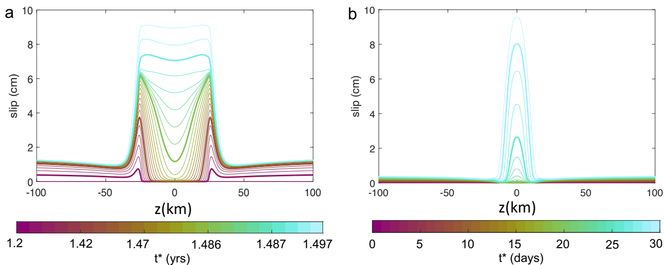
Figure S2. Profiles of slip accumulation during induced SSE of representative models under (a) type I (Figure S1) and (b) type II (Figure 6) perturbation. t^* is the time since the start of the perturbation. Note that we only consider the pressurization phase, when most of the slip accumulates. For (a), time contours are not regularly spaced, as shown in the colorbar. Contours for (b) are every \sim 1 day.
