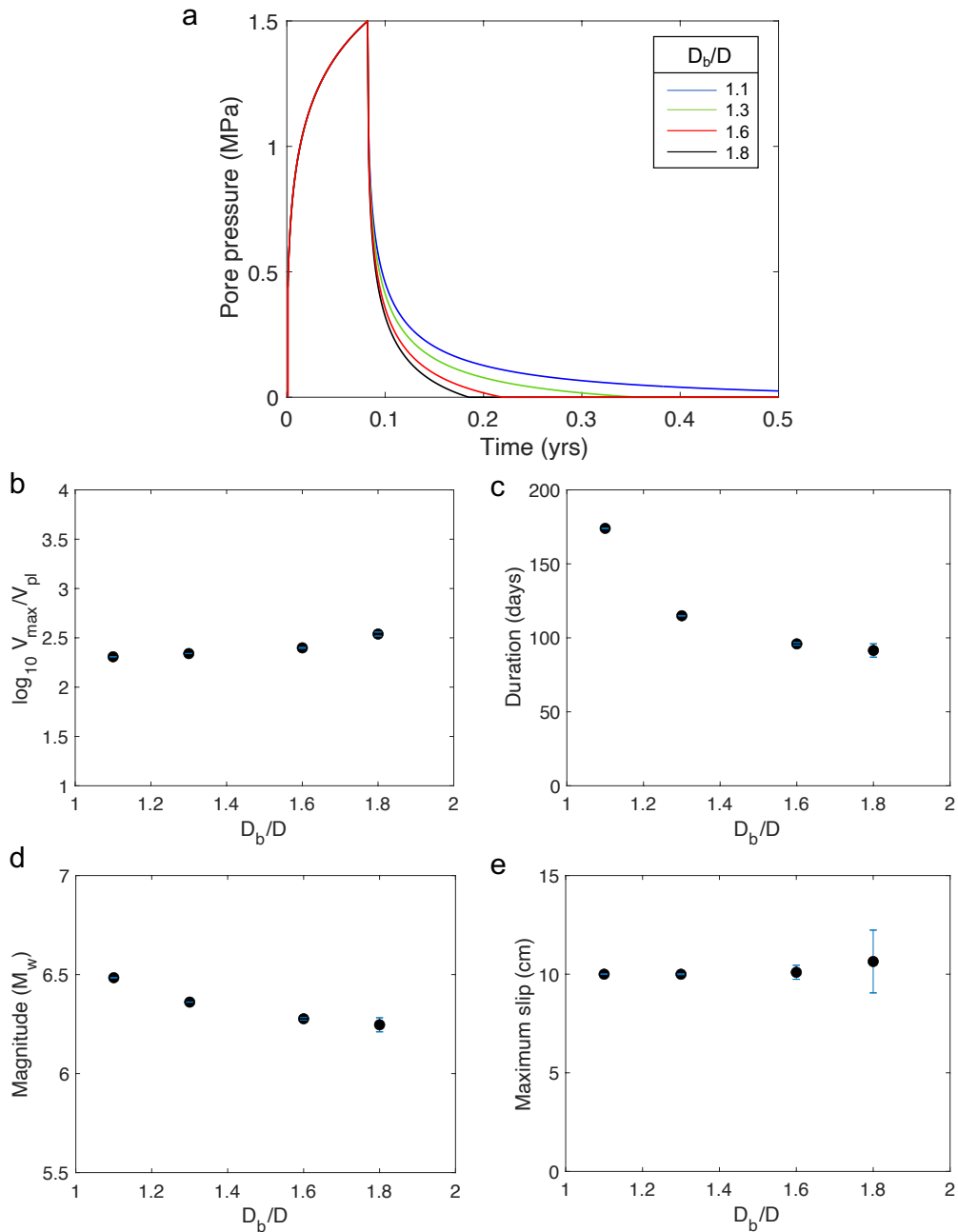
Figure S4. (a) Evolution of pore pressure at the fault center r = r_0 for different values of D_b/D . Perturbation parameters are D = 25 \text{ m}^2/\text{s} , t_{inj} = 30 \text{ days} and \Delta p_{\max} = 1.5 \text{ MPa} . Case with D_b/D = 1.6 corresponds to the perturbation parameters of the representative model for type II perturbation (Table 2). (b–e) Average SSE properties: (b) normalized maximum slip rate, (c) duration, (d) magnitude and (e) maximum slip, shown as a function of D_b/D , assuming all other parameter constant. Vertical lines indicate standard deviation. Perturbation parameters are the same as given in (a).
