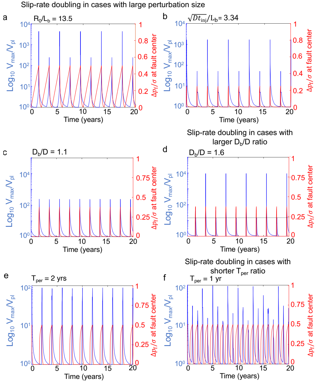
Figure S5. Examples of simulations to illustrate the cases in which slip-rate doubling emerged during the explorations in Figures 7 and 9. (a–f) Temporal evolution of V_{max}/V_{pl} (blue line) and \Delta p_f/a\sigma at the fault center (red line). Simulation cases under (a) type I perturbation with \Delta p_{max}/a\sigma=100 and R_0/L_b=13.5 ( R_0=56.25 km) and (b) type II perturbation with \Delta p_{max}/a\sigma=75 and \sqrt{Dt_{inj}}/L_b=3.34 ( \sqrt{Dt_{inj}} = 11.4 km, D = 75 m 2 /s, t_{inj} = 30 days). (c–d) Simulations with \sqrt{Dt_{inj}}/L_b = 2.74 (with D = 50 m 2 /s and t_{inj} = 30 days) and \Delta p_{max}/a\sigma = 75 , but different D_b/D : (c) 1.1 and (d) 1.6. Dashed black line in (d) indicates the peak velocity of the slow-velocity SSE. (e–f) Simulation cases with \sqrt{Dt_{inj}}/L_b \sim 3 ( D = 10 m 2 /s, t_{inj} = 0.5 yr) and \Delta p_{max}/a\sigma = 100 , but different perturbation period: (e) 2 yrs and (f) 1 yr. Model parameters are as given for shallow Hikurangi SSEs for (a) to (d), and for deep SSEs for (e) and (f) (Table 1).
