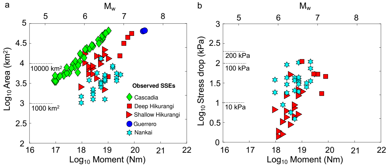
Figure S7. Source properties of observed SSEs from Cascadia (Michel et al., 2019), deep and shallow Hikurangi (Ikari et al., 2020), Guerrero (Radiguet et al., 2012) and Nankai (Takagi et al., 2019) subduction zones. (a) Moment-Area. (b) Moment-stress drop. Note that only stress drops from Nankai and Hikurangi SSEs were constrained by observations. To define the stress drop of deep Hikurangi SSEs from Ikari’s (2020) catalog, we calculated the average stress drop between the different stages of each event.
